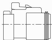
18.71mm W x 23.89mm H x 29.92mm L DT06-3S-EPO6
