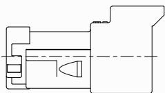
21.14mm W x 24.71mm H x 44.65mm L DT04-3P-E005
