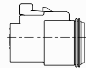
18.37mm W x 23.731mm H x 28.40mm L DT06-3S
