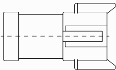
36.45mm W x 25.40mm H x 47.19mm L DT04-08PA-E005
