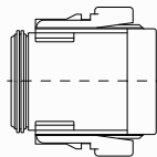
37.21mm W x 22.15mm H x 32.44mm L DT06-08SA-EPO6
