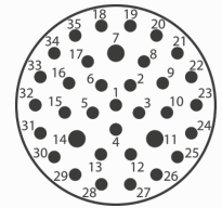
24-35 3 x size 16, 32 x size 20
