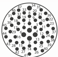
24-47 5 x size 16, 42 x size 20
