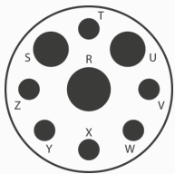
24-9 1 x size 4, 2 x size 8, 6 x size 12
