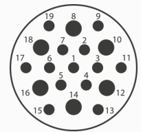
24-19 6 x size 12, 13 x size 16
