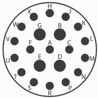
24-21 4 x size 12, 17 x size 16
