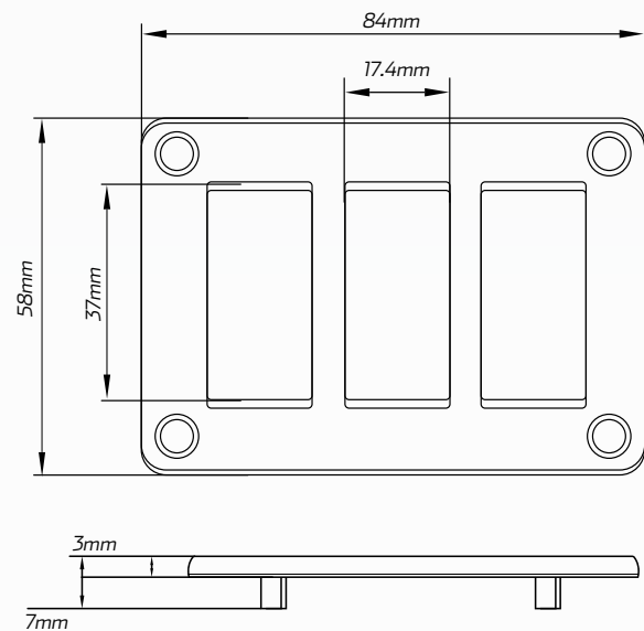
• Dimension diagram is based of #QVSWHLB3
